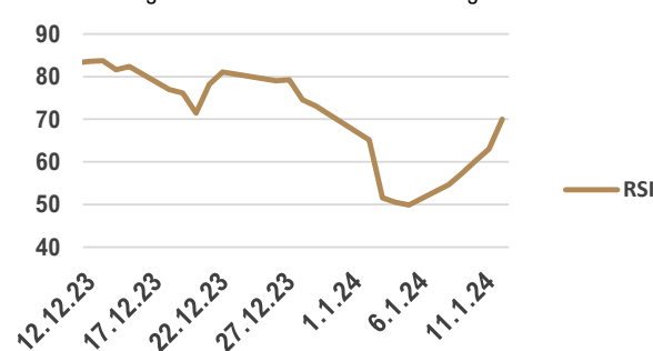
Figure 5: RSI is exactly 70
