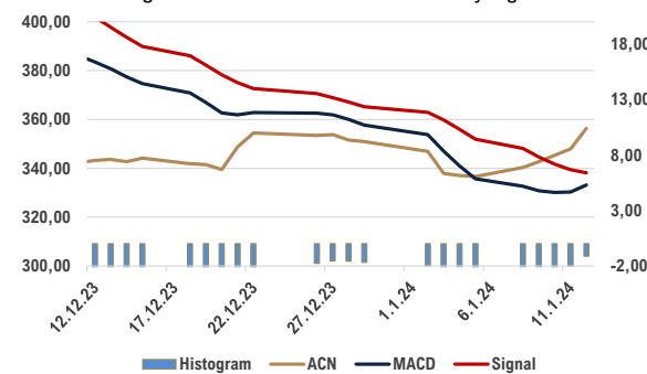
Figure 4: MACD line is below the signal line
