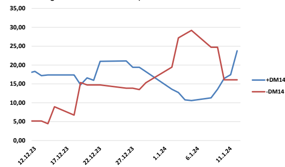
Figure 2: DMI indicates a buy signal
